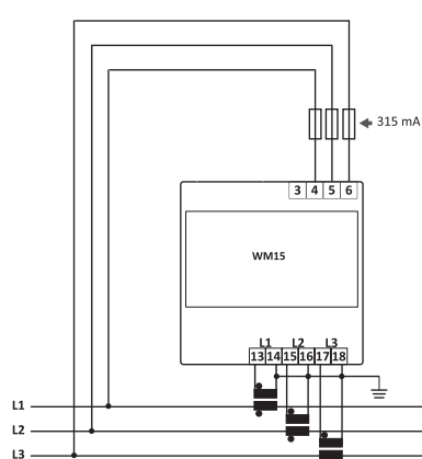
Fig. 10 Three-phase without neutral (3-wire)
