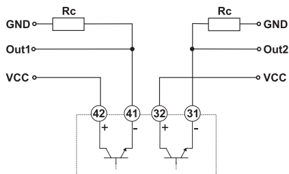
Fig. 26 Static outputs, VCC reference
